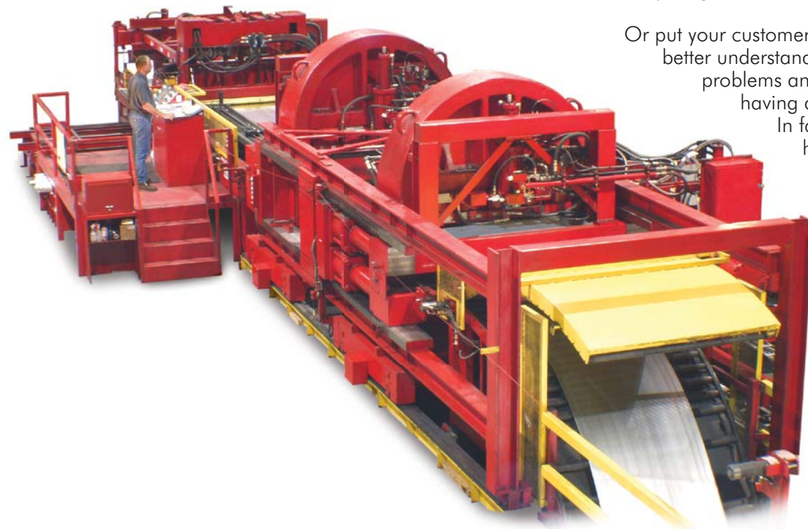
TMW's Stretcher Leveler gets material flatter than temper pass, leaving it able to achieve 1/4 of ASTM A568 Table 15 tolerances after laser or plasma cutting.
