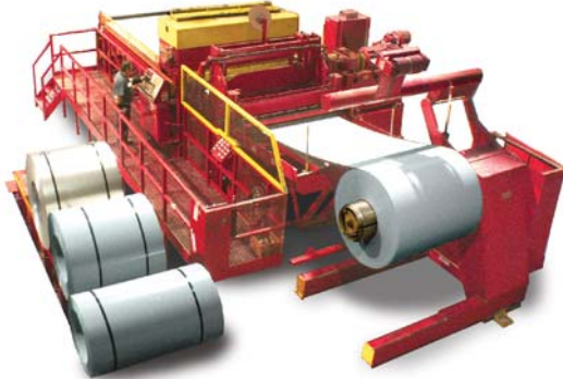
Multi-Cut Blanking of pre-painted coils
